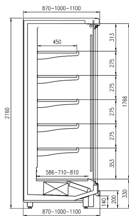
VENEZIA H216 Ecovision
